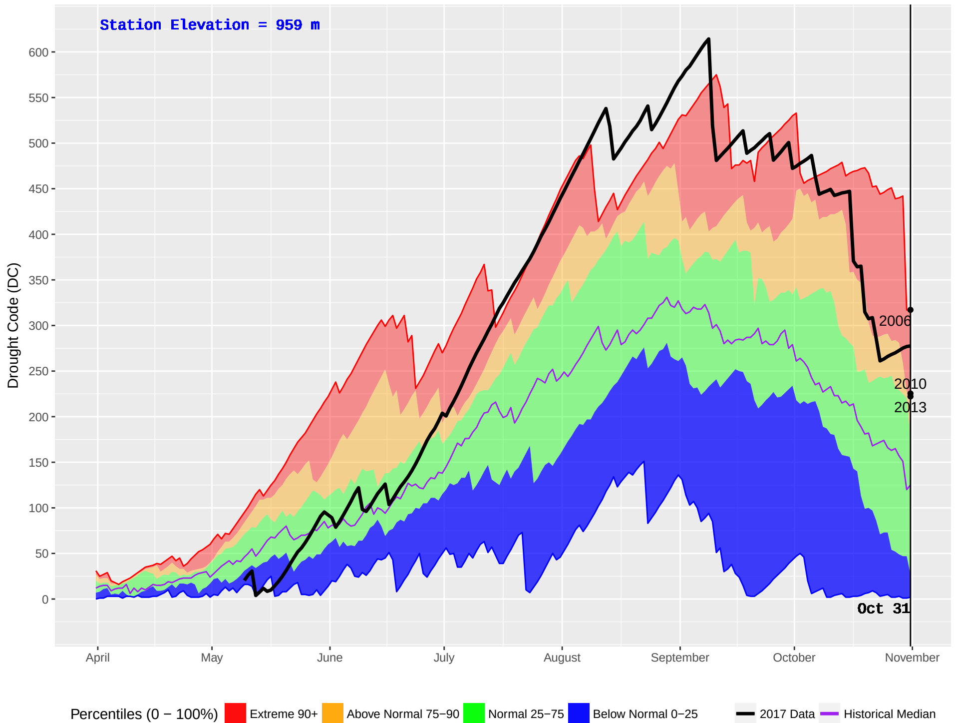
WELLS GRAY (266) : Historical (1994–2016) and Current (2017) Noon Drought Code (DC)
