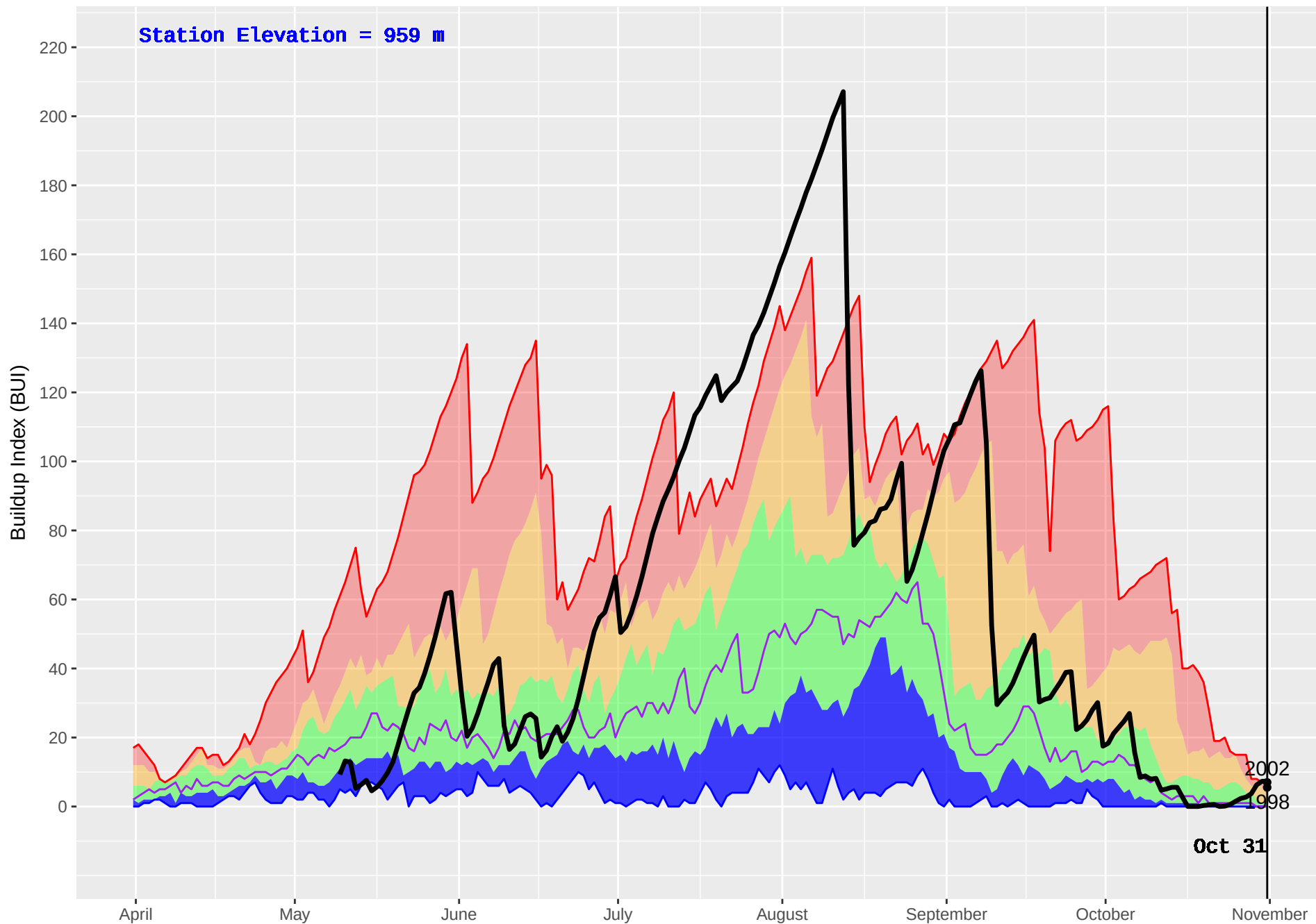
WELLS GRAY (266) : Historical (1994–2016) and Current (2017) Noon Buildup Index (BUI)
