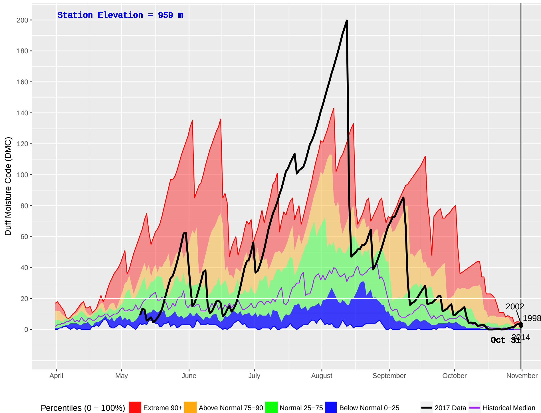
WELLS GRAY (266) : Historical (1994–2016) and Current (2017) Noon Duff Moisture Code (DMC)
